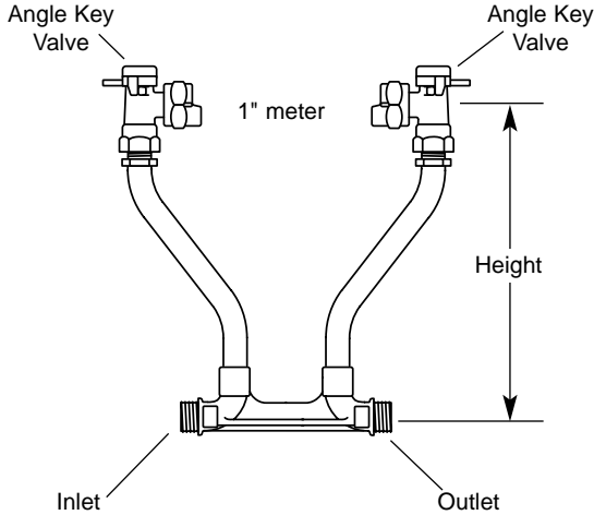
Male Threads for Pack Joint Assemblies (PJAx-4x)
