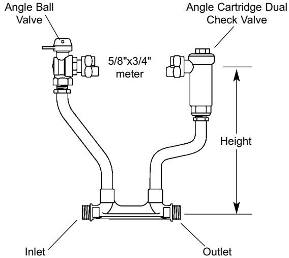
Male Threads for Pack Joint Assemblies (PJAx-1x)
