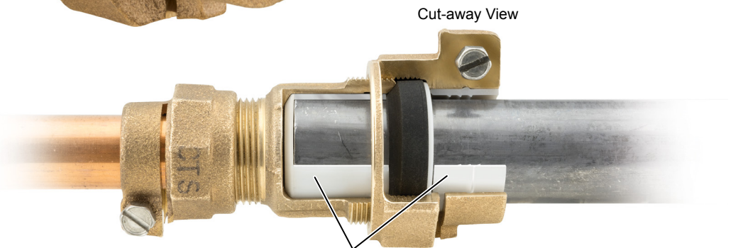
Permanently installed plastic gripper ring and sleeve liner prevent direct contact between lead pipe material and other metallic water system components
