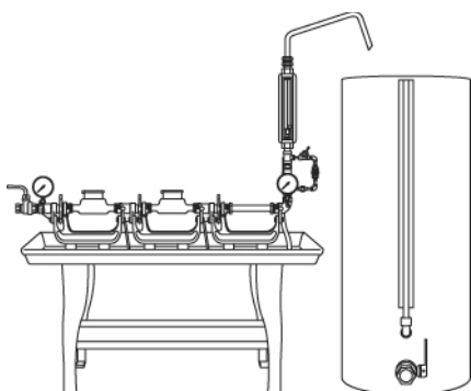
Standard Test Bench (with manual clamping)
