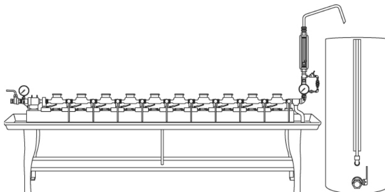
Indianapolis Test Bench (with hydraulic clamping)
